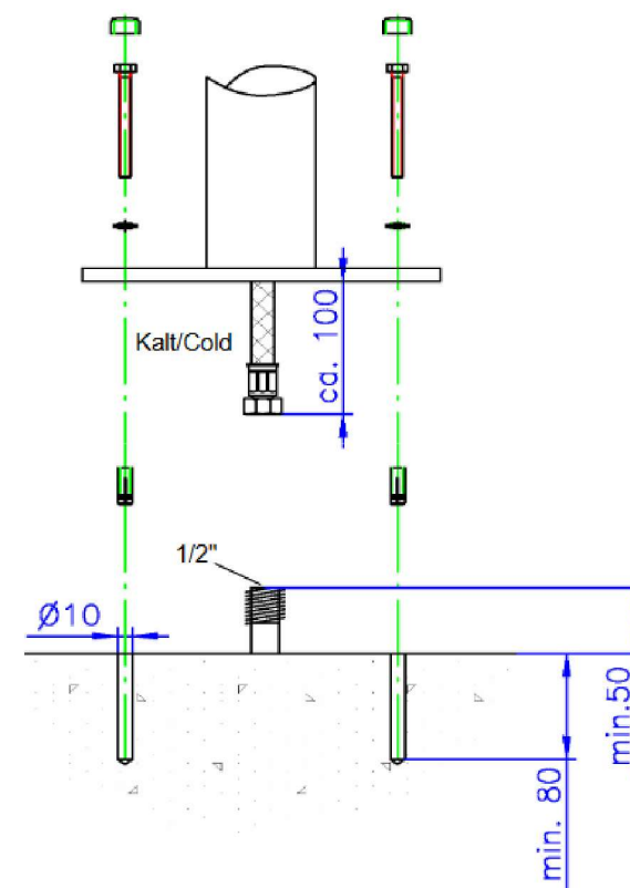
Detail X
