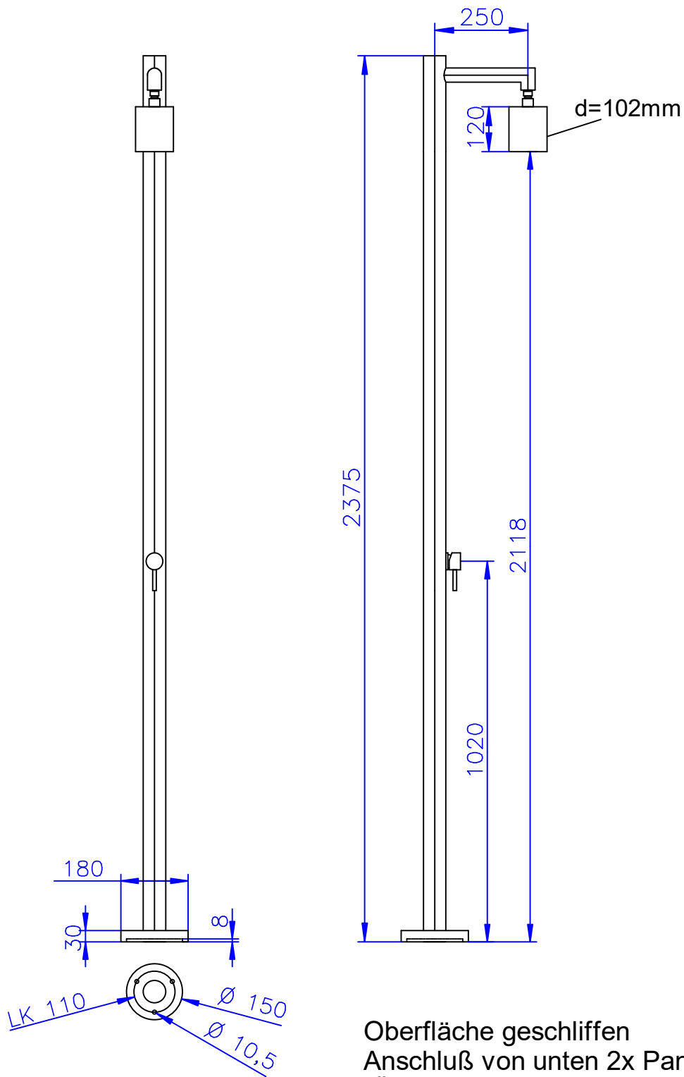
Detail Brausekopf
